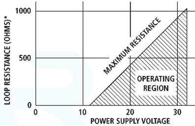
* Loop resistance=Wire res.+Receiver res.
